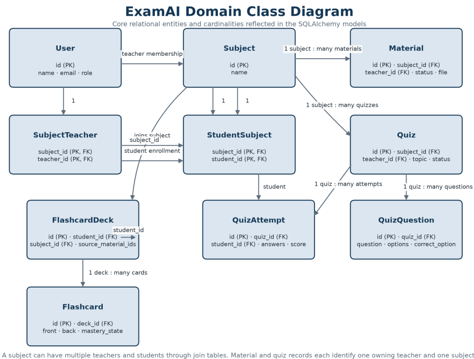
Figure 7.2: Class diagram
